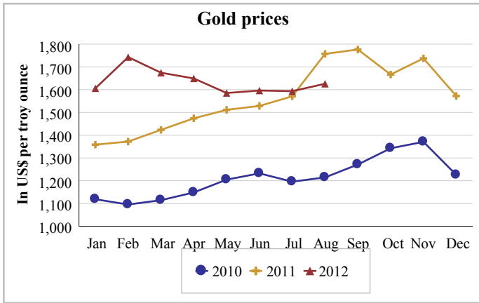
Chart 7.9
